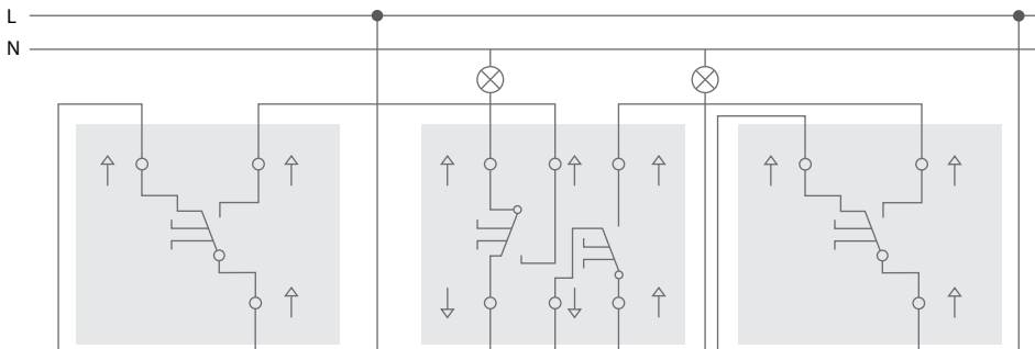
1-GANG TWO-WAY SWITCH
