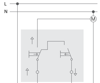
2-GANG BLIND SWITCH
