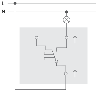
1-GANG TWO-WAY SWITCH
