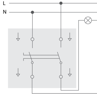
1-GANG 2 POLE SWITCH
