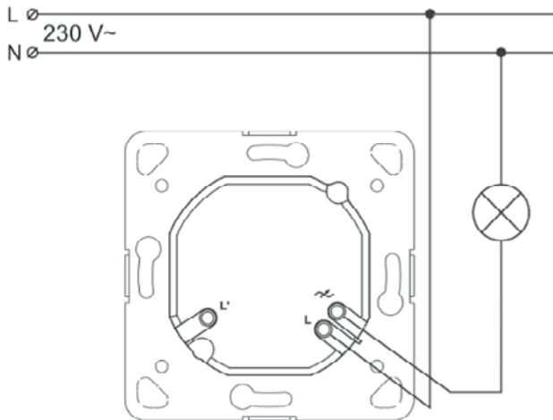
Typical 1-way circuit connecting diagram
