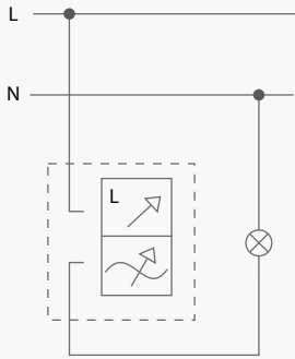
For incandescent, halogen and dimmable compact 220V lamps
