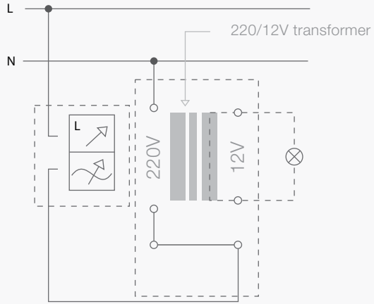
For halogen 12V lamps, connected via transformer
